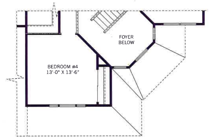
ZENITH TERRACE - SECOND FLOOR PLAN
