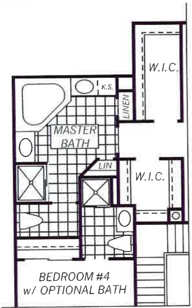
SECOND FLOOR PLAN OPT. FULL BATH IN 4TH BEDROOM
