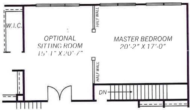
SECOND FLOOR PLAN OPT. EXPANDED MASTER SUITE
