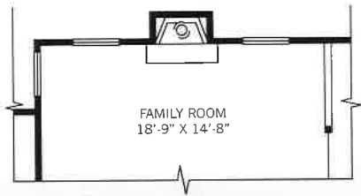
FIRST FLOOR PLAN OPT. FIREPLACE
